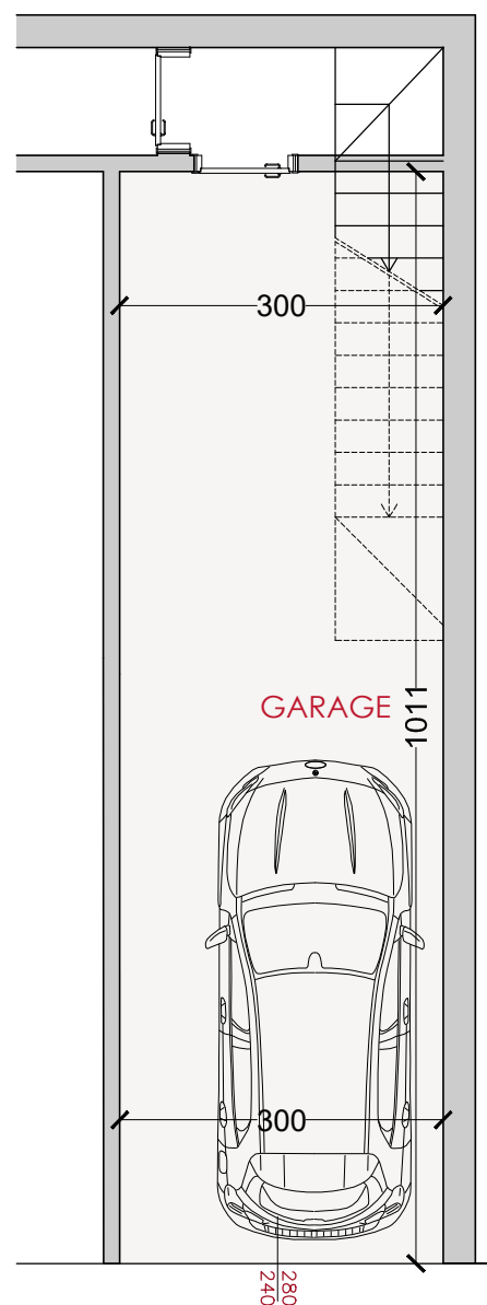
Piano interrato
