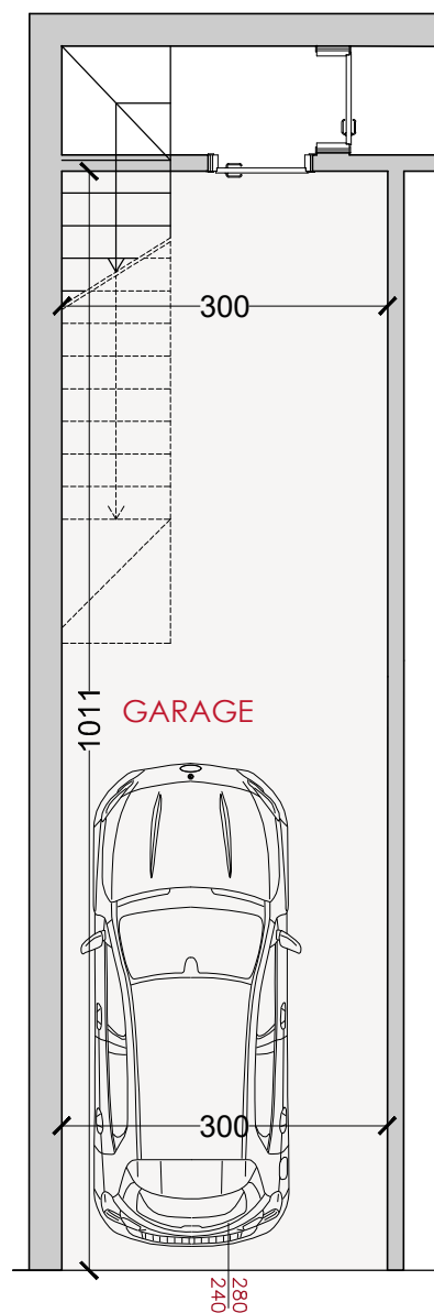
Piano interrato
