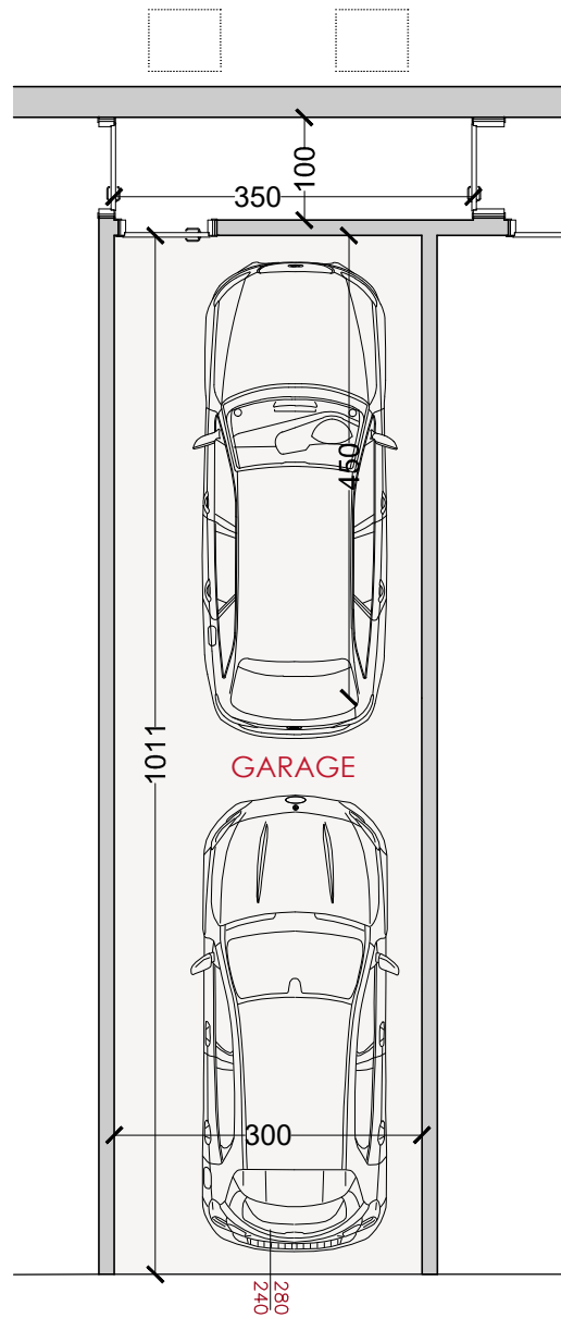
Piano interrato
