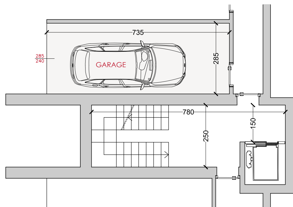
Piano interrato
