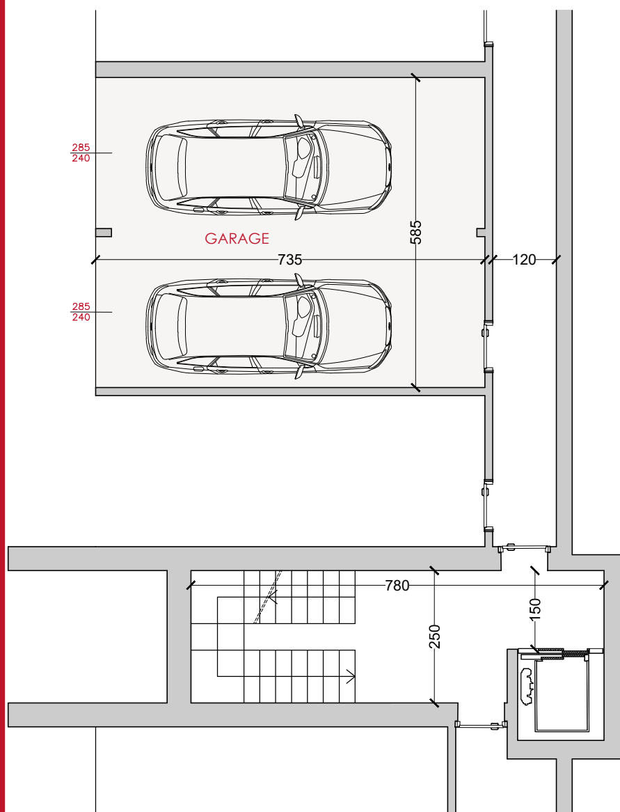
Piano interrato
