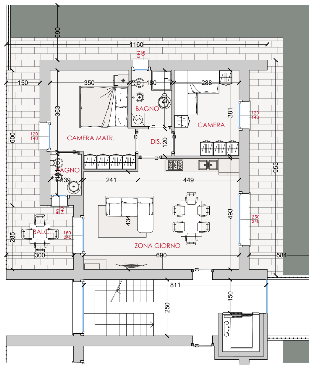
Piano terra
